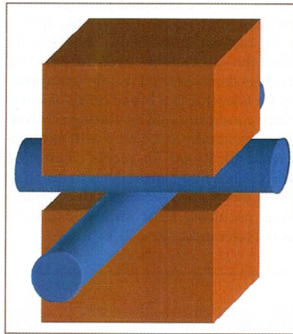
Fig. 1 — 'Single' and 'double knot' cross wire welds.
