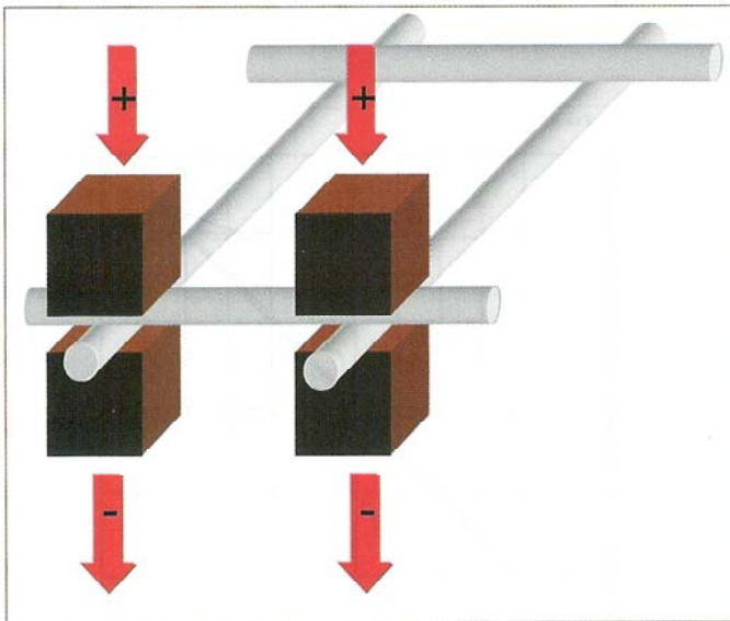
Fig. 4 — Direct welding.
